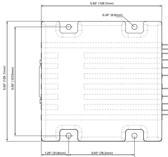
FIGURE 14. FBL2360 top view and dimensions
