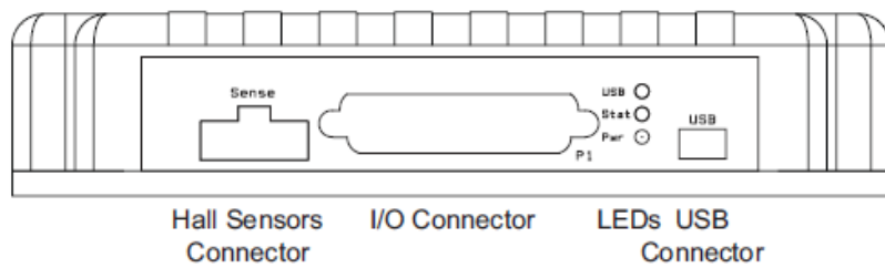
FIGURE 1. FBL2360 front view
