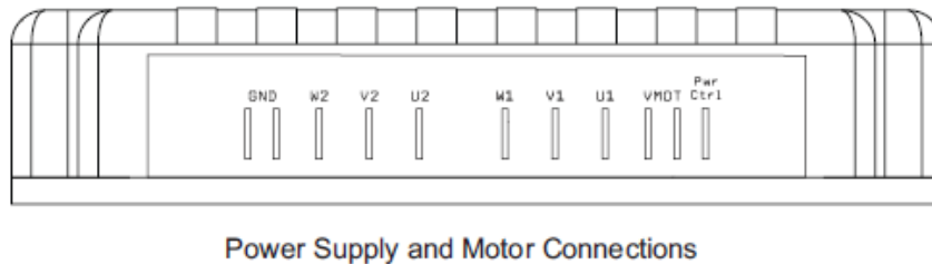
FIGURE 2. FBL2360 rear view
