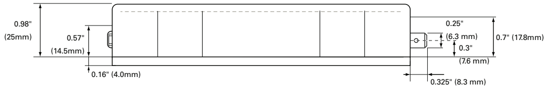
FIGURE 13. FBL2360 side view and dimensions
